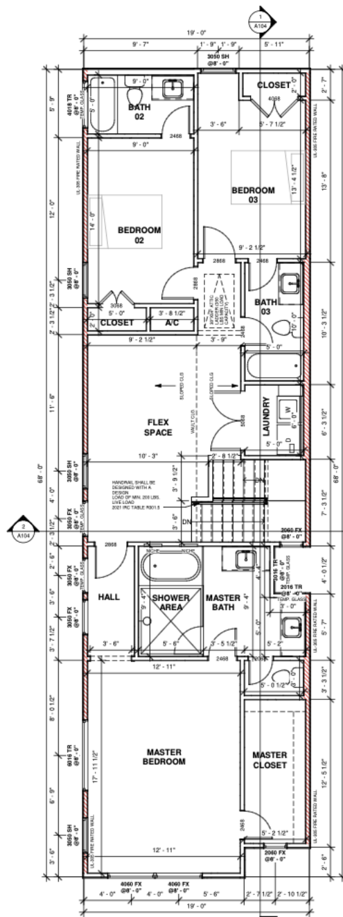
2 2ND FIN. FLOOR TYPE-A 1/4" = 1'-0"
