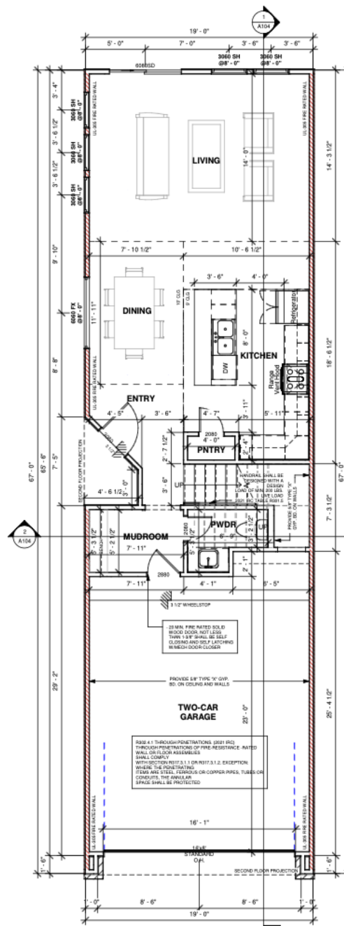
1 1ST FIN. FLOOR TYPE-A 1/4" = 1'-0"
